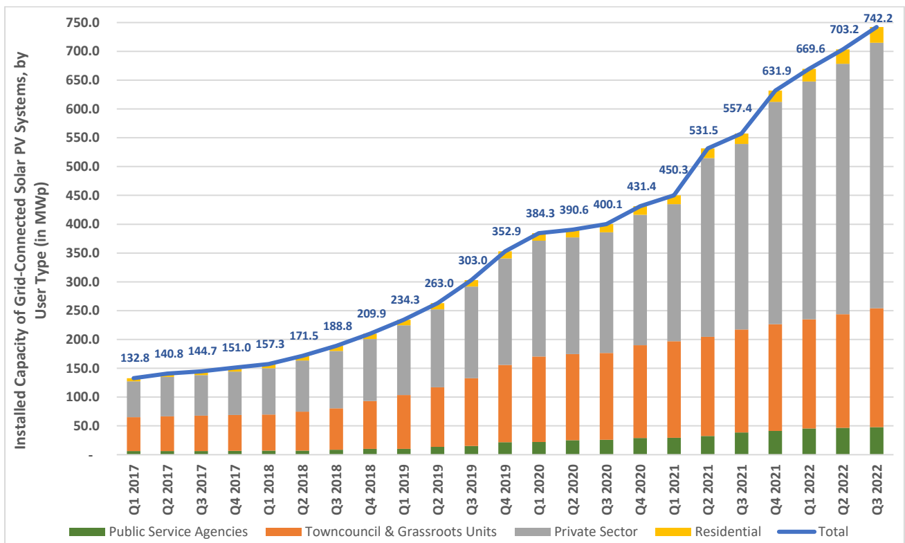
Figure 1: Installed Capacity of Grid-Connected Solar PV Systems (in MWp), 1Q 2017 – 3Q 2022 (as at end of each quarter)
