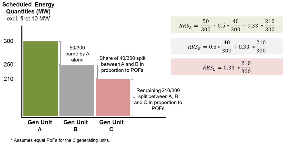
Figure 2: Illustration of Modified Runway Model
